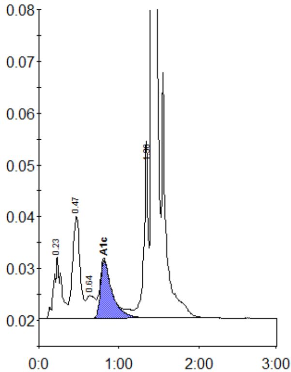
Peak table - ID: 10668543
